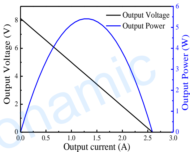
The chart for output voltage and output power Vs output current under Th=300 °C and Tc=30 °C
